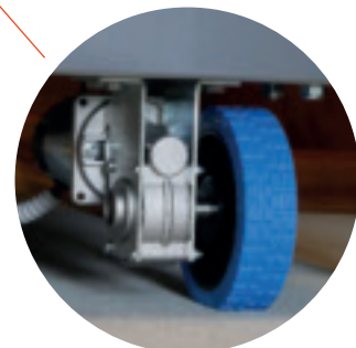
Long-life electric motor with integrated motorized wheel \varnothing 150\text{mm}
